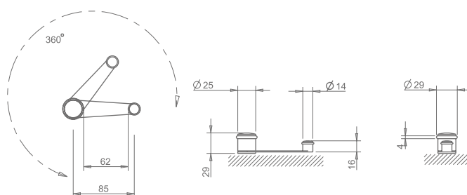
Double door stopper with fastener door
