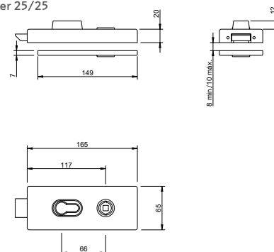
Door lock for glass European cylinder 25/25
