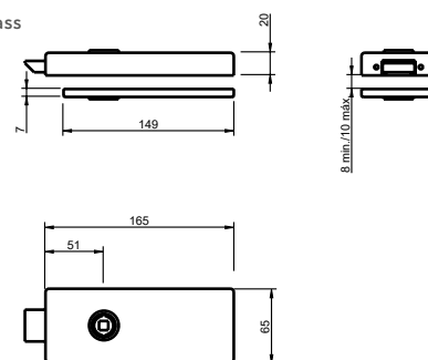
Door lock for glass European cylinder 25/25
